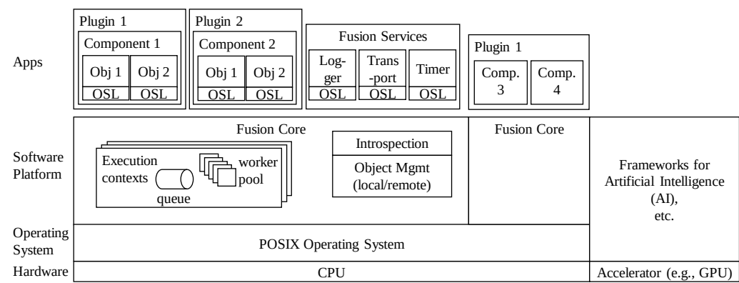
■ Figure 2 An example of a software system built with Fusion: Multiple identical instances of the Fusion engine (Fusion core) run in operating system processes and host components, which are implemented through Fusion objects ( Obj ). Execution contexts are used to process messages and services for users are provided. Artificial Intelligence (AI) frameworks already abstract accelerators and are running alongside Fusion.
