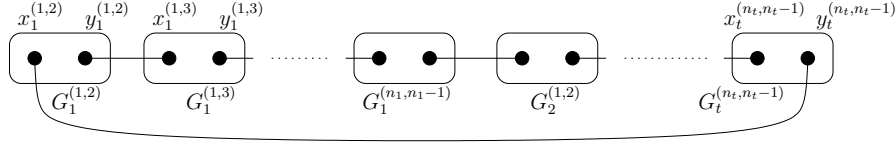
■ Figure 1 The construction of G' .
