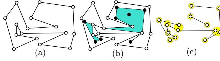
■ Figure 1 (a) A simple polygon P . (b) Eight points in the interior of P (solid dots); their geodesic hull is a weakly simple polygon P' with 14 vertices. (c) A perturbation of P' into a simple polygon.
