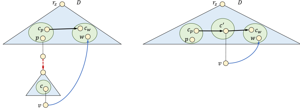
■ Figure 5 Before the insertion of (x, y) , edge (v, w) corresponds to the shortcut edge (p, w) of \hat{G}_{r_z} , and is stored in out(c_p) . An auxiliary component with canonical vertex c is affected by the insertion of (x, y) and is merged into a component with canonical vertex c' ( c' = c if the component is moved without merging with another component). Now c' becomes the canonical vertex of the nearest ancestor of v in D_z , and edge (v, w) is stored as a shortcut edge in out(c') .
