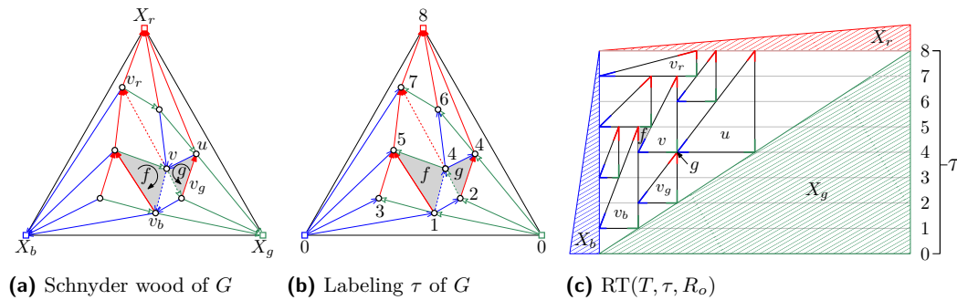
Figure 3 (a) A Schnyder wood T of a plane triangulation G ; the edges connecting v with vertices v_r , v_g , and v_b are dashed. (b) Graph \text{DAG}_r(T) with ADT-labeling \tau . (c) An RT-representation of G constructed from T , \tau , and an RT-representation R_o of the outer face.
