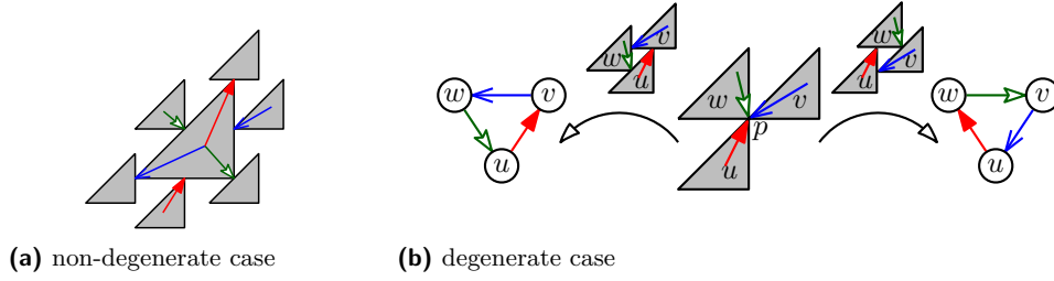
■ Figure 2 From an RT-representation to a Schnyder wood.
