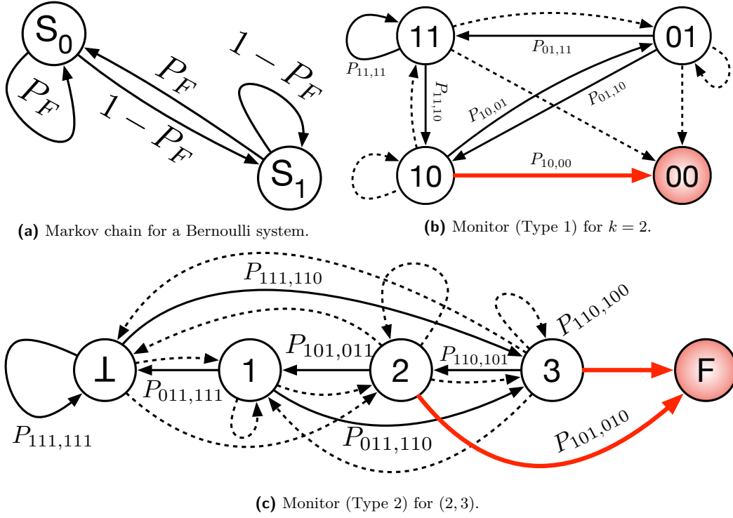
Figure 2 PMC approach. In inset (b), P_{x_1x_2, y_1y_2} is a shorthand for transition probability P'(q, q') where states q and q' have labels L'(q) = x_1x_2 and L'(q') = y_1y_2 , respectively. In inset (c), P_{x_1x_2x_3, y_1y_2y_3} is a shorthand for P'(q, q') , where states q and q' correspond to execution histories x_1x_2x_3 and y_1y_2y_3 , respectively. Since the Type 2 monitor is represented more concisely, the node labels in inset (c) are not equal to the execution histories, e.g., label “3” indicates an execution history of “110” where the latest iteration has failed. In insets (b) and (c), transitions with zero probability are marked with dashed arrows, and states in Bad(1, 2) and Bad(2, 3) are colored red.
