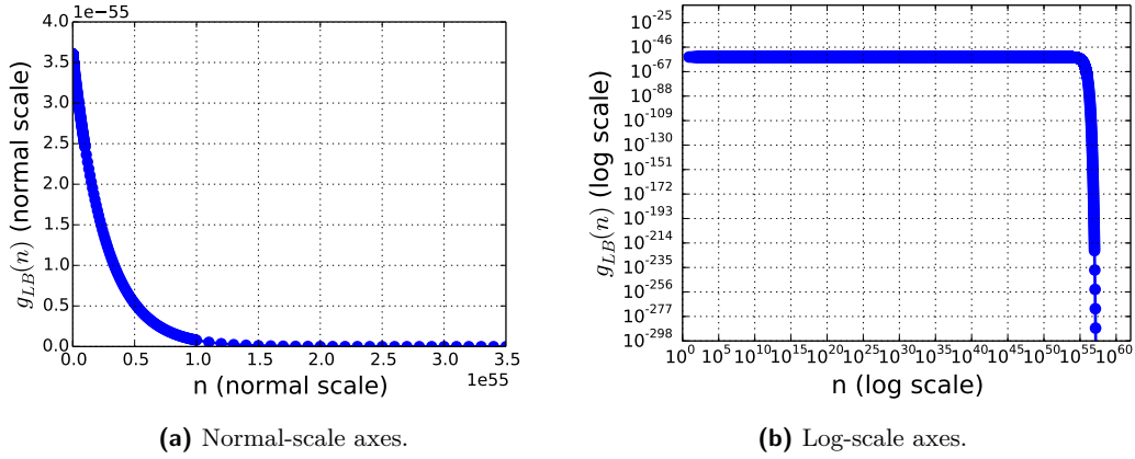
■ Figure 3 Sampling points g_{LB}(d_0), g_{LB}(d_1), \dots, g_{LB}(d_D) for m = 3 , k = 10 , P_F = 10^{-7} , and T = 10 ms in (a) normal scale and (b) log scale. In this example, D = 5050 and d_D = 9.90 \times 10^{57} .
