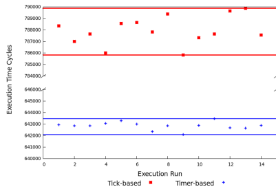
■ Figure 4 Execution under tick-based and interval-timer time management.
